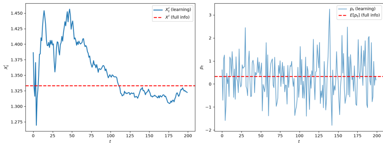
Fig. 128.3: equilibrium trade and prices over time
