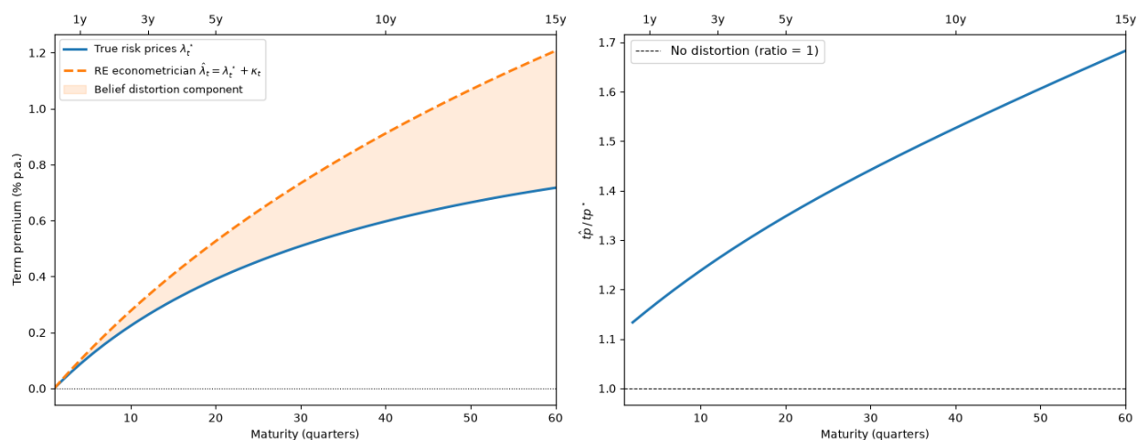
Fig. 130.5: True vs. distorted-belief term premiums and overstatement ratio
