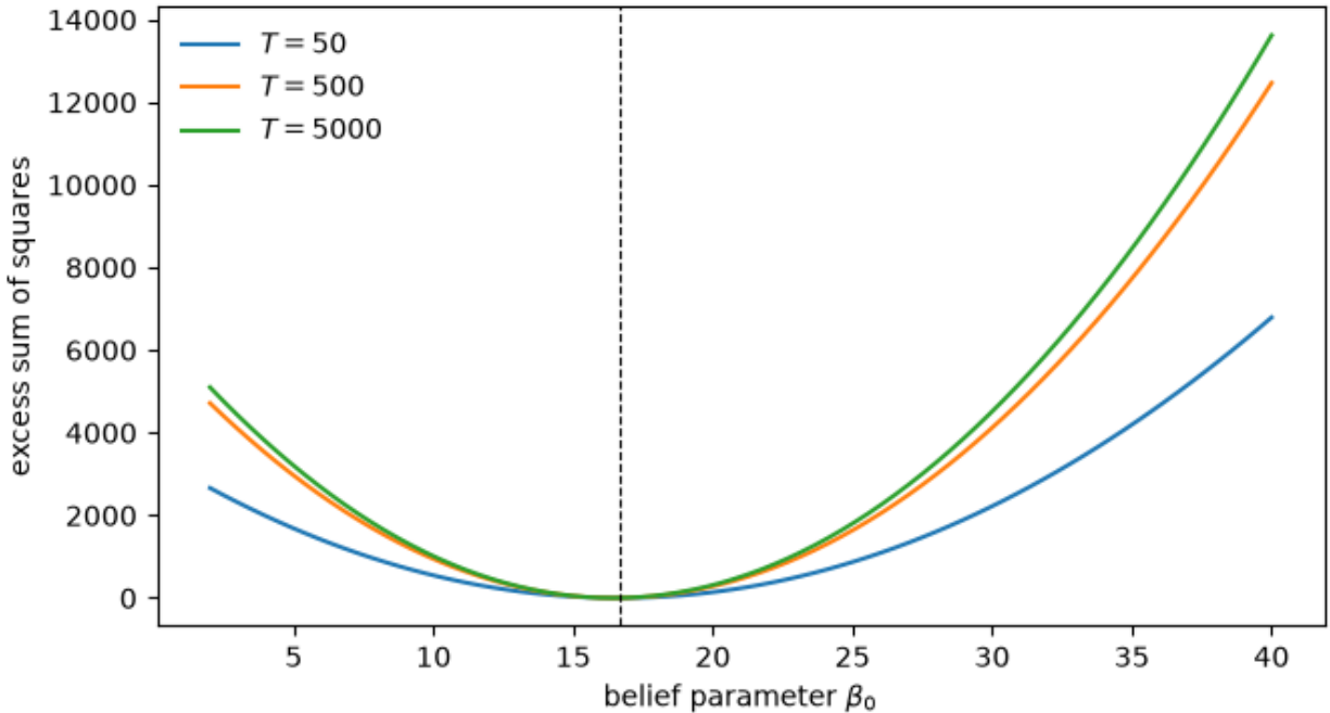
Fig. 95.2: Information about the belief parameter stops accumulating
