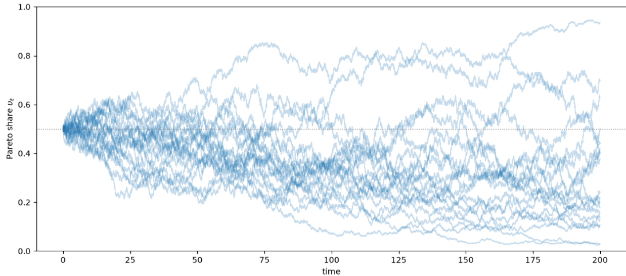
Fig. 35.4: Pareto-share paths in the separable benchmark
