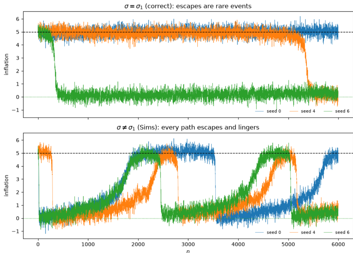
Fig. 104.4: Escapes are rare under the correct error variance and pervasive under Sims's misallocation
