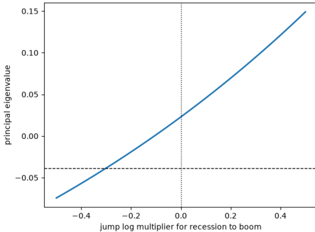
Fig. 132.2: Jumps and the long-run growth rate
