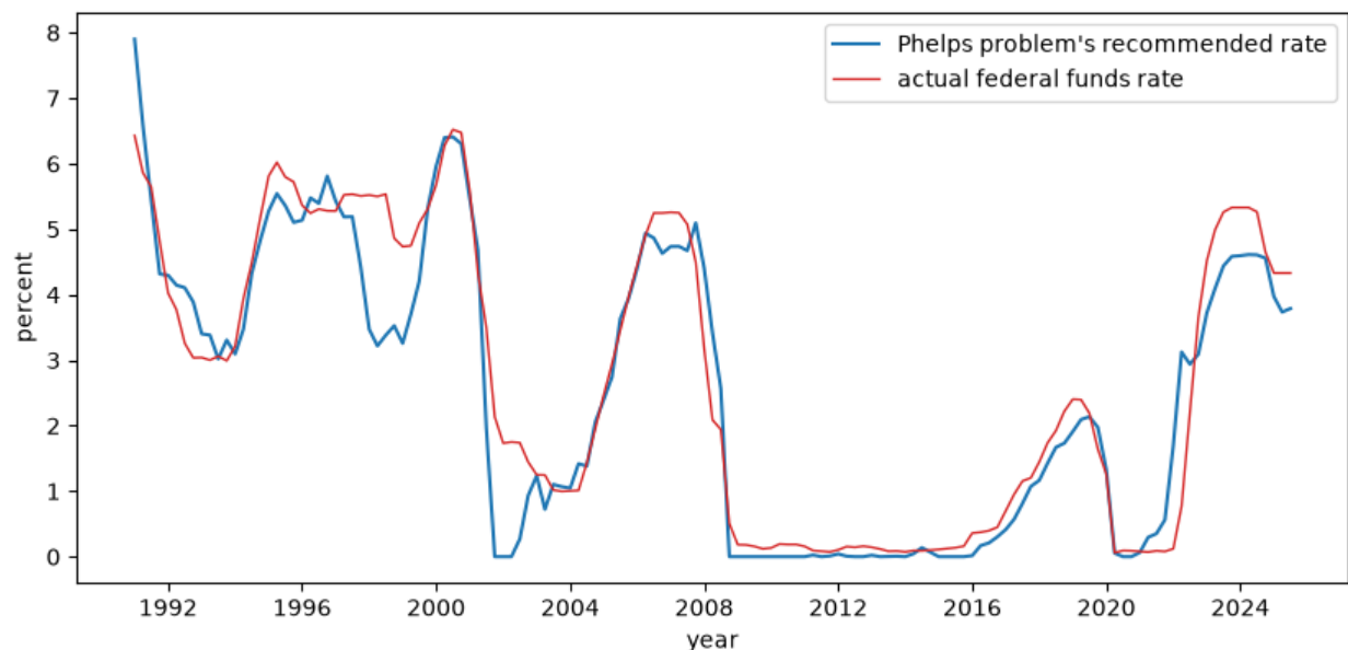
Fig. 105.2: The belief-driven Phelps rule against the actual federal funds rate
